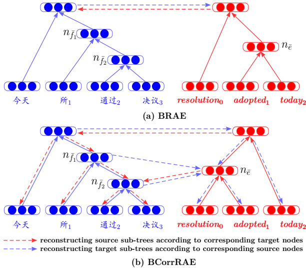
Figure 1: BRAE vs BCorRAE models for generating of a bilingual phrase (“今天 所 通过 决议”, “ resolution adopted today ”) with word alignments (“0-2 2-1 3-0”). The subscript number of each word indicates its position within phrase. Solid lines depict the generation procedure of phrase structures, while dash lines illustrate the reconstruction procedure from one language to the other. In this paper, the dimensionality of vector d in all figures is set to 3 for better illustration.
