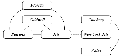
Figure 1: Mention context graph for the Caldwell example.
